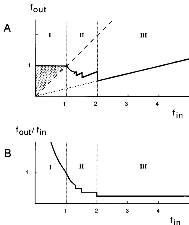
FIGURE 10 Frequency transformation in a beaded nerve fiber. (A) A plot of the relative output frequency as a function of input frequency for a beaded nerve fiber. The broken line represents a normal cylindrical nerve fiber where input equals output. Note that when f_{in} < f_{rev} (region I) that the input frequency is amplified such that f_{out} = f_{rev} . For the case in which f_{rev} < f_{in} < 2f_{rev} (region II), the output frequency decreases nonlinearly. When f_{in} > 2f_{rev} (region III), then f_{in} is linearly reduced by a fraction of 1/4. (B) A plot of the transformation coefficient versus input frequency f_{in} . Again, when f_{in} < f_{rev} , the coefficient is >1 , indicating amplification. Between f_{rev} \rightarrow 2f_{rev} , the input frequency is nonlinearly filtered and has a value between 1 and 0.25. When f_{in} > 2f_{rev} , the coefficient becomes linear at a value of 0.25.
