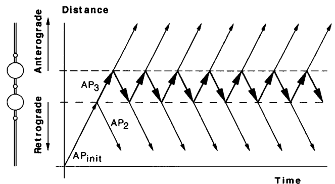
FIGURE 7 A pair of reflecting beads along a nerve fiber. In this case a single action potential ( AP_{init} ) entering a region of two reflecting beads (a reverberator) can produce recurrent generation of both anterograde and retrograde nerve impulses. The resultant frequency is the intrinsic frequency of the reverberator. Thus a single action potential can be multiplied many times before reaching its destination.
